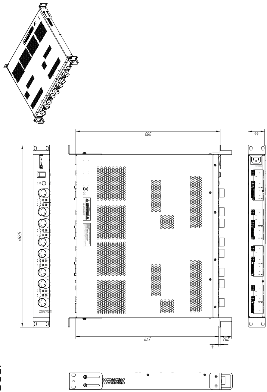
Ecler AURA-8L150 Mechanical Diagram
